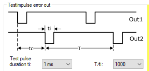
Abb. 4-8: Testimpulse
