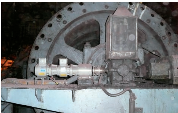
After: More precise signals because of robust combination of bearing block and heavy duty encoders.
